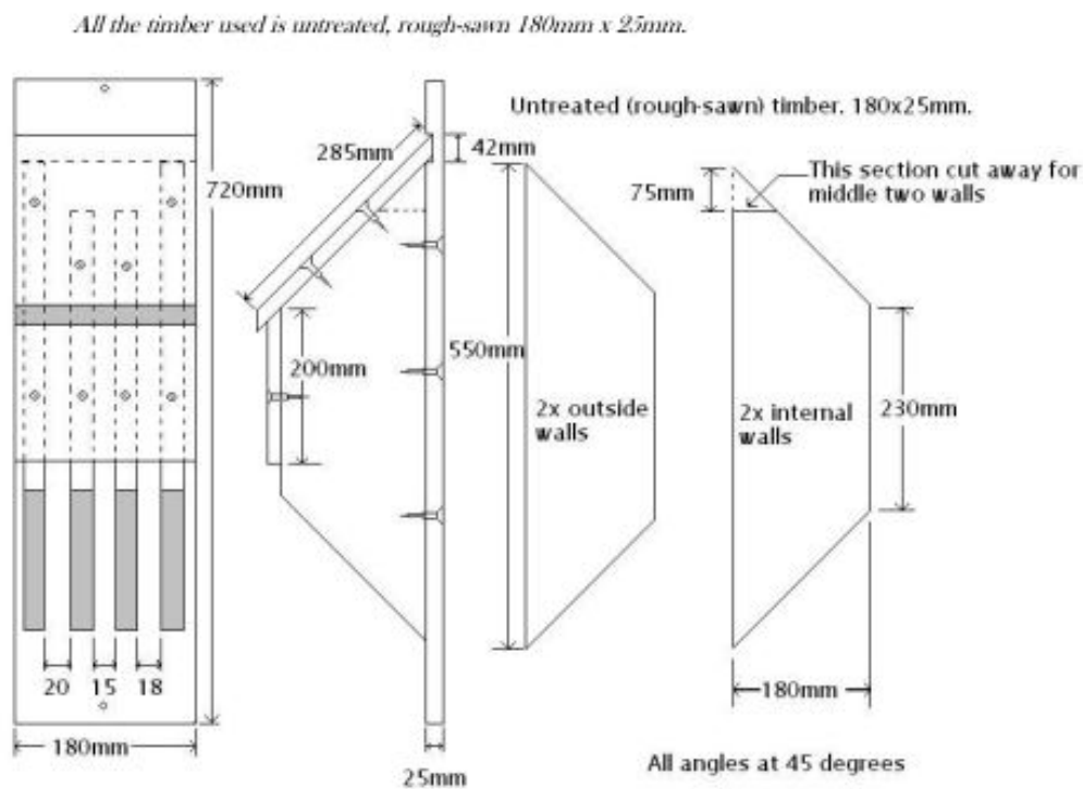
Figure 1-1 Schematic of the slot box design
